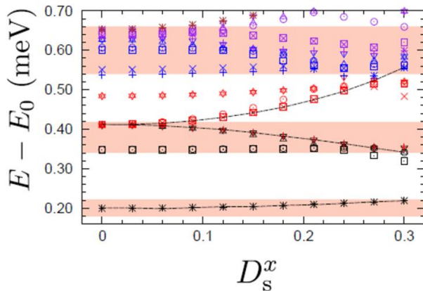
Fig.2: Energy spectrum for D_u^z = 0.12 , J_1/J_2 = -3.1 , J'/J_2 = 0.47 , J_2 = 37.5 (K). Excited levels from the ground state are depicted by the symbols + , \times , \square , \circ , \triangle , and \nabla . Three shaded bands represent the areas for the first three low-energy peaks in inelastic neutron-scattering spectra of \text{Rb}_2\text{Cu}_2\text{Mo}_3\text{O}_{12} .
