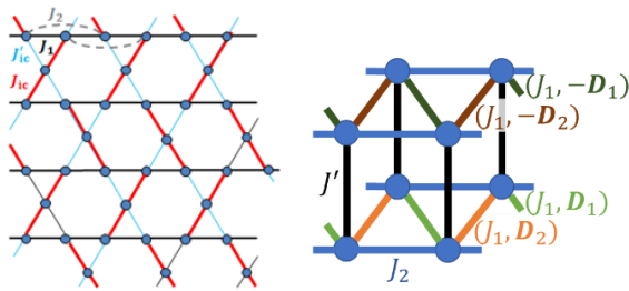
Fig.1: Left: Distorted kagome lattice network of spin exchange interactions proposed for the volborthite. Right: Coupled ferromagnetic- J_1 antiferromagnetic- J_2 frustrated spin ladder for \text{Rb}_2\text{Cu}_2\text{Mo}_3\text{O}_{12} . The Dzyaloshinski-Moriya vectors are taken as \mathbf{D}_1 = J_1(D_s^x, 0, D_u^z) and \mathbf{D}_{1'} = J_1(-D_s^x, 0, D_u^z) in one spin chain, and by -\mathbf{D}_1 and -\mathbf{D}_{1'} in the other chain.
